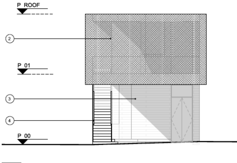
Image 1.4 – Pavilion. South Elevation
