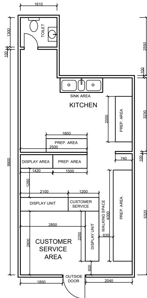
FLOOR PLAN SCALE 1:100
